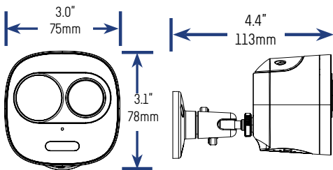
Camera with Wall Mount
